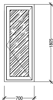
DETAIL J1
