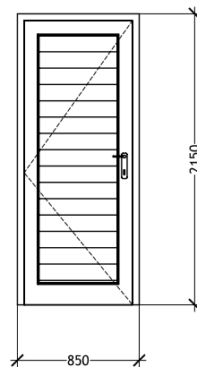
DETAIL P2
