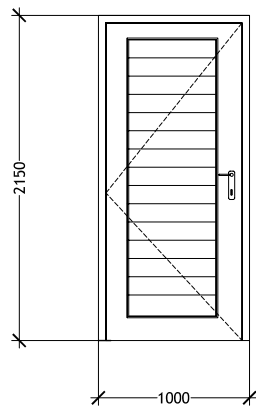
DETAIL P1
