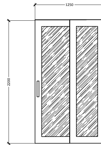
RENCANA PJ2 SLIDING
